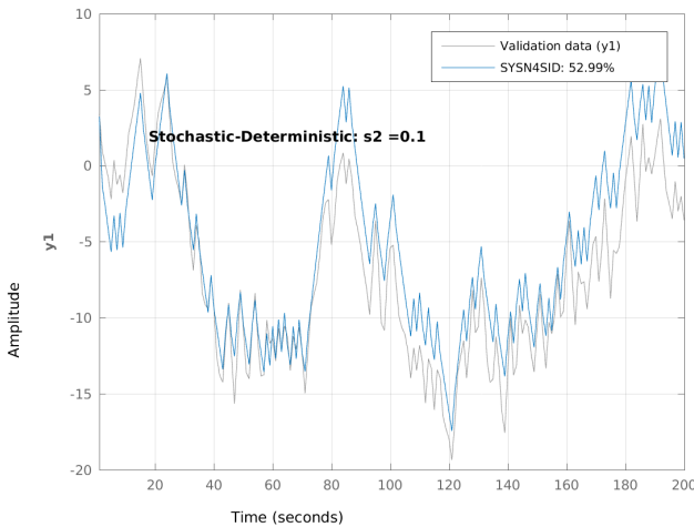
FIGURE 12: Combined simulation with s2 = 0.1
