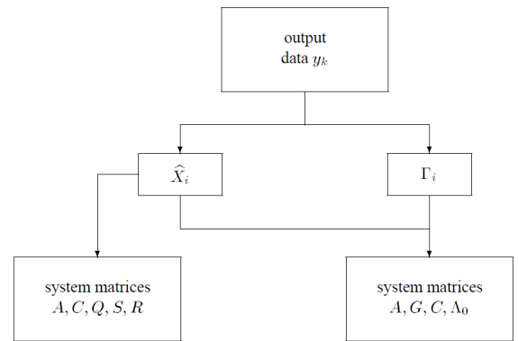
FIGURE 5: An overview of the stochastic subspace method.
